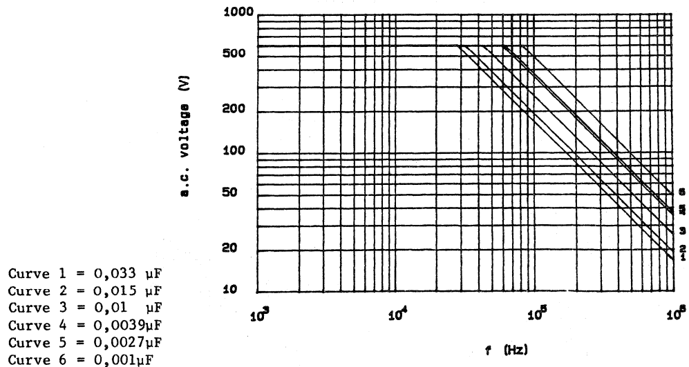
Fig. 10: a.c. voltage (r.m.s. value) as a function of frequency at T_{\text{amb}} < 85^{\circ}\text{C} for U_{\text{Rdc}} = 2000\text{V}
