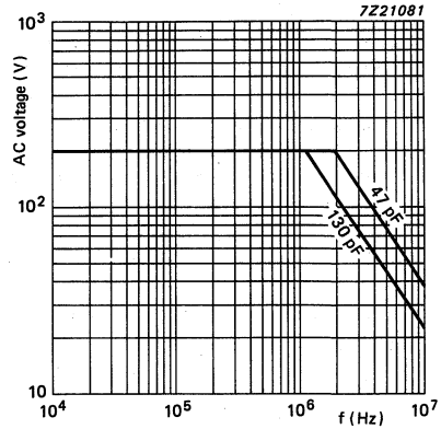
Fig. 13 Maximum a.c. voltage (r.m.s. value as a function of frequency at T_{amb} \leq 70^\circ\text{C} , for U_R = 630\text{ V} .
