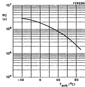
Fig. 12 RC product as a function of ambient free air temperature; typical curve.
