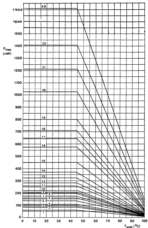
Fig. 15 : Maximum dissipation as a function of ambient free air temperature.
