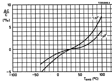
Fig. 3 : Capacitance as a function of ambient free air temperature; typical curve.
