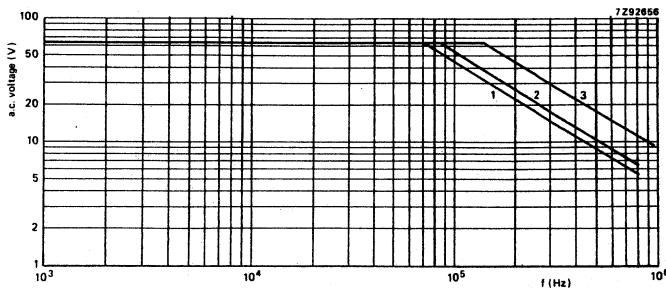
Fig. 3 Maximum a.c. voltage (r.m.s. value) as a function of frequency at T_{amb} < 70^{\circ}C , for U_R = 160V .
