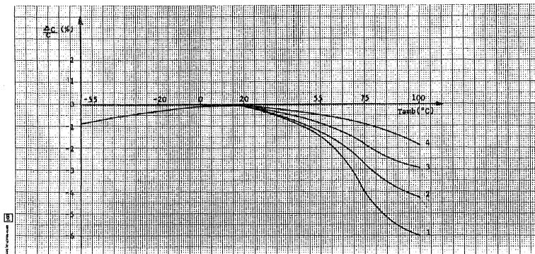
Fig. 6 : Capacitance as a function of ambient free air temperature, measured at 1kHz, typical curves. 1. 100V series 2. 250V series 3. 400V series 4. 630V series
