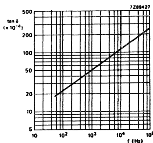
Fig. 4 : Tan delta as a function of frequency, typical curve
