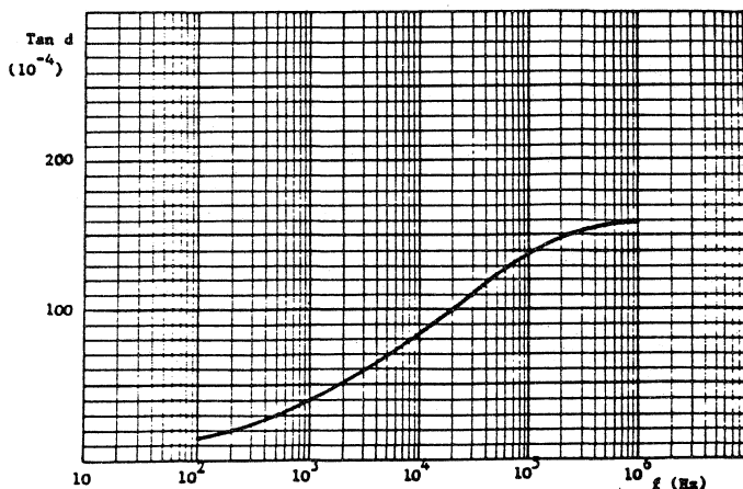
Graph : \text{Tan}_\Delta as a function of frequency; typical curve.
