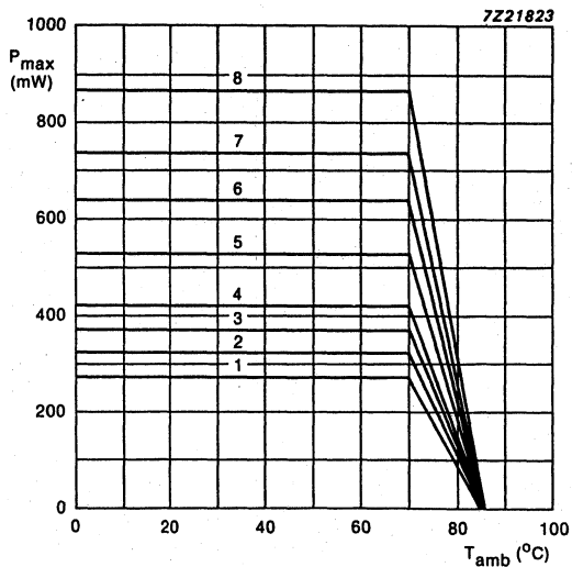
Fig.14 : Maximum permissible power dissipation as a function of ambient free air temperature, at various capacitor dimensions.
