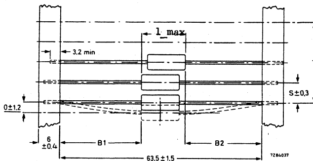
Fig. 10 |B1-B2| = \max. 1,4\text{mm} , for dimension l_{max} see tables 1 to 4
