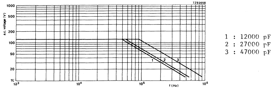
Fig. 4 Maximum a.c. voltage (r.m.s. value) as a function of frequency at T_{amb} \leq 70^{\circ}C , for U_R = 250V .
