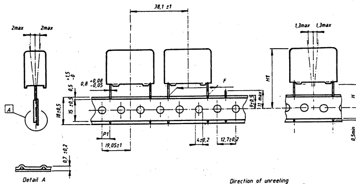
Capacitors with pitch P = 22,5 or 27,5mm, Fig. 3
