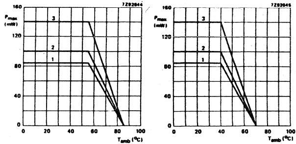
Fig. 8 Maximum permissible power dissipation as a function of ambient free air temperature.
