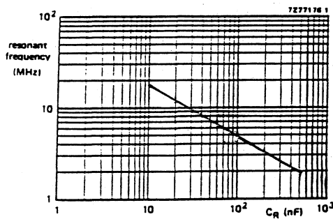
Fig. 8 Resonant frequency as a function of rated capacitance.
