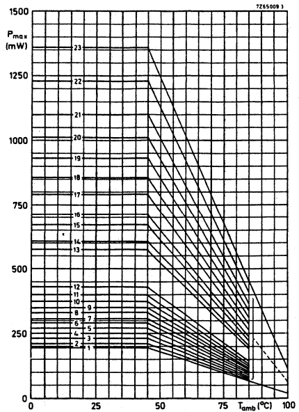
Fig. 7 Maximum permissible power dissipation as a function of ambient free air temperature.
