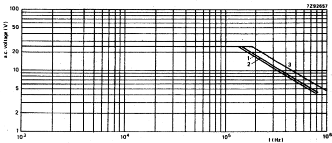
Fig. 2 Maximum a.c. voltage (r.m.s. value) as a function of frequency at T_{amb} < 55^{\circ}C , for U_R = 63V .
