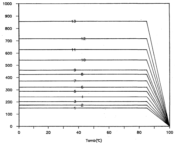
Pmax (mW) as a function of temperature
