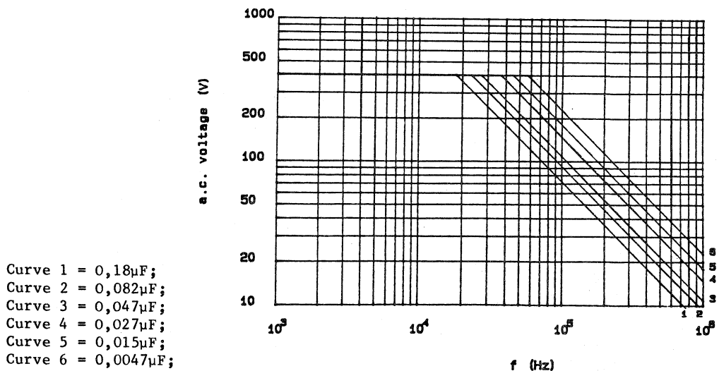
Fig. 8 a.c. voltage(r.m.s. value) as a function of frequency at T_{amb} \leq 85^{\circ}C , for U_{Rdc} = 1000V .
