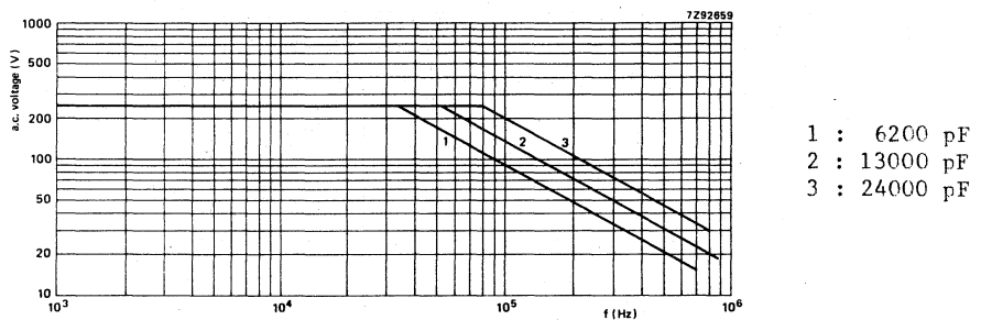
Fig. 5 Maximum a.c. voltage (r.m.s. value) as a function of frequency at T_{amb} \leq 70^{\circ}C , for U_R = 630V .
