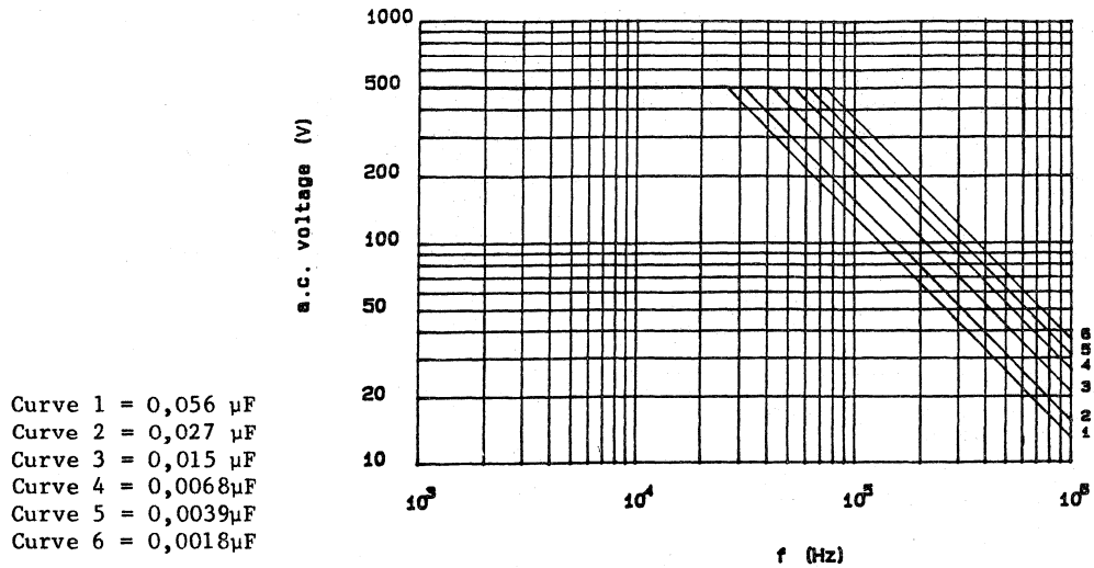
Fig.9 : a.c. voltage (r.m.s. value) as a function of frequency at T_{\text{amb}} < 85^{\circ}\text{C} for U_{\text{Rdc}} = 1600\text{V}
